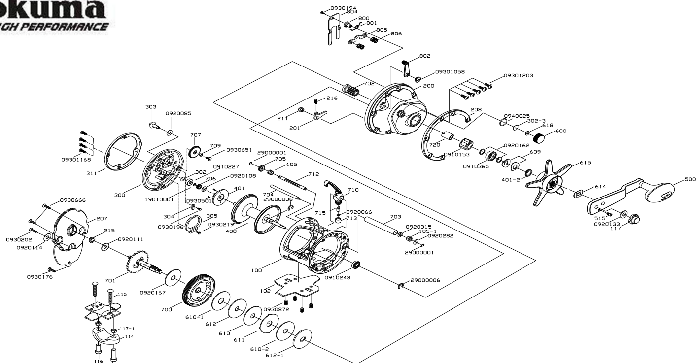
CT-30L PARTS LIST
