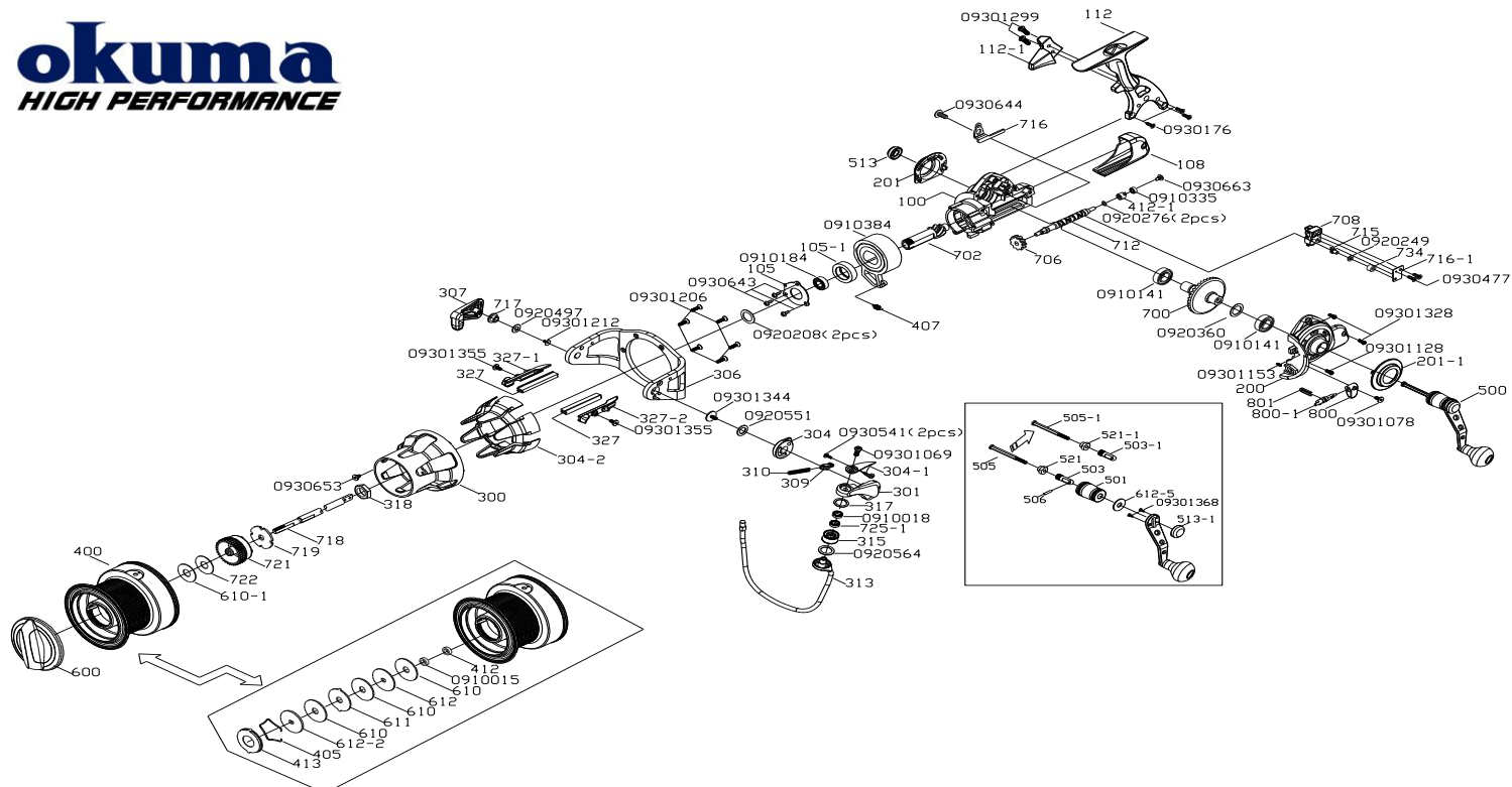
TXS-60 PARTS LIST
