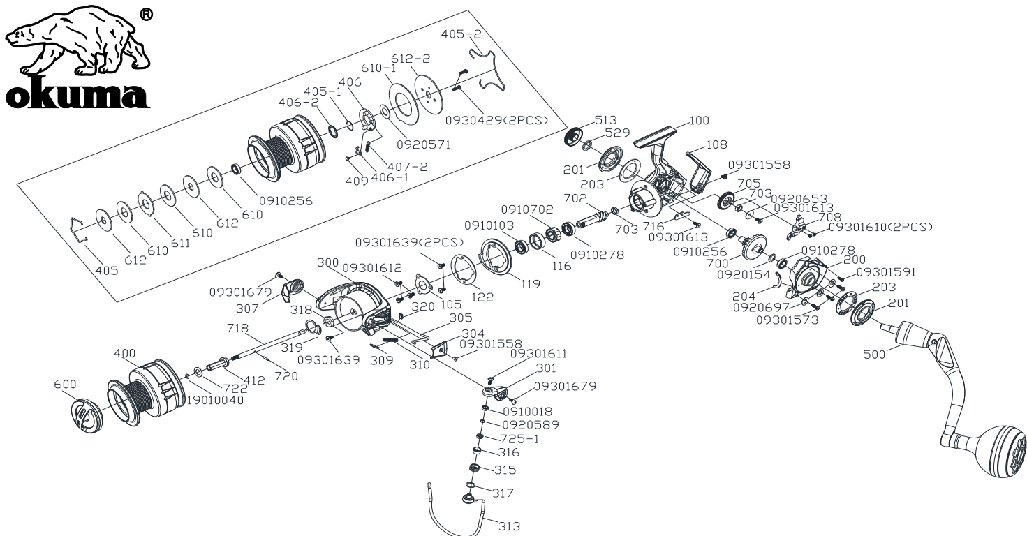
SA-4000HA 零件清單
