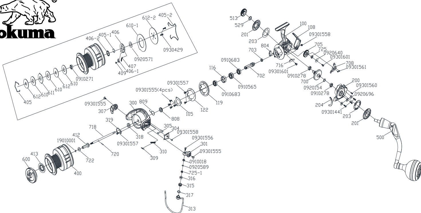
SA-10000A 零件清單
